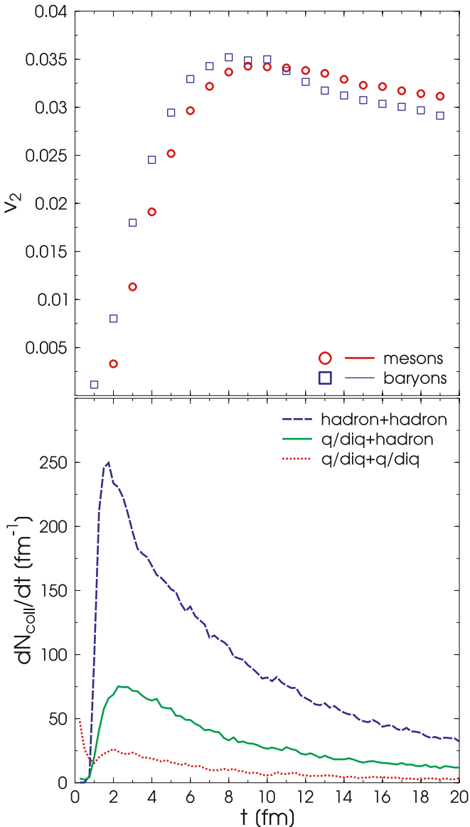
Fig. 1. UrQMD calculation for Au + Au interactions at \sqrt{s_{NN}} = 200 GeV. Top: meson and baryon v_2 versus time at midrapidity. Bottom: collision rates as a function of time for hadron+hadron (dashed line), hadron+quark/di-quark (full line) and quark/di-quark+quark/di-quark (dotted line)
