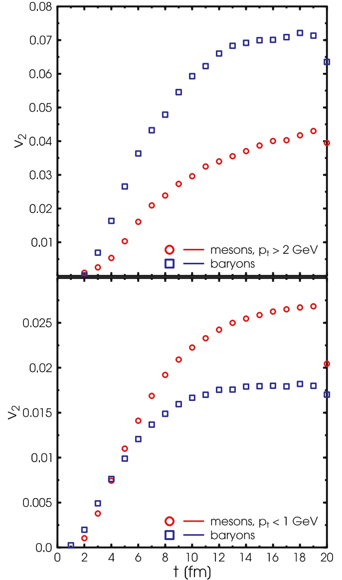
Fig. 2. UrQMD calculation for Au + Au interactions at \sqrt{s_{NN}} = 200 GeV. Bottom: meson and baryon v_2 versus time at midrapidity and p_T \leq 1 GeV/c. Top: meson and baryon v_2 versus time at midrapidity and p_T \geq 2 GeV/c
