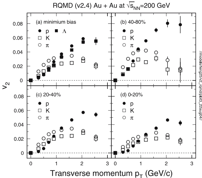
Fig. 5. RQMD results of \pi , K , p , and \Lambda v_2 from Au + Au collisions at \sqrt{s_{NN}} = 200 GeV. (a) Minimum bias collisions: at about p_T \sim 1.2 GeV/c, baryon and meson v_2 are crossing each other; (b) 40%–80%; (c) 20%–40%; (d) 0%–20%
