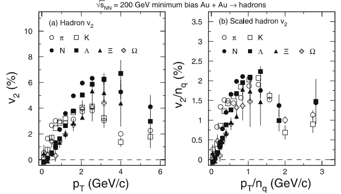
Fig. 6. (a) Hadron v_2 from minimum bias Au + Au collisions at \sqrt{s_{NN}} = 200 GeV; (b) scaled hadron v_2 results are shown. The n_q refers to the number of constituent quarks. Symbols represent results from the UrQMD (v2.2) model for various hadron species. At low p_T/n_q \leq 0.5 GeV/c, \pi does not follow the scaling perhaps caused by the resonance decay [17]. In the higher p_T region, K meson seems to fall off the scaling curve due to the comparatively small hadronic cross sections in the model
