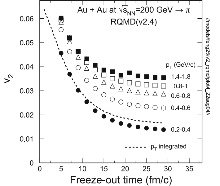
Fig. 4. Elliptic flow ( v_2 ) of pions from RQMD versus their freeze-out time for several p_T windows for minimum bias Au + Au collisions at \sqrt{s_{NN}} = 200 GeV. The dashed-line represents the p_T integrated distribution
