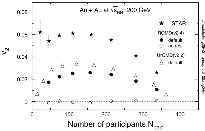
Fig. 3. Charged hadron v_2 versus the number of participating nucleons in Au + Au interactions at \sqrt{s_{NN}} = 200 GeV. Experimental data [34, 35] from the 4-particle cumulant method is shown as stars. RQMD results are depicted by filled circles (full calculation) and open circles (without rescattering). The UrQMD calculations are shown as open triangles
